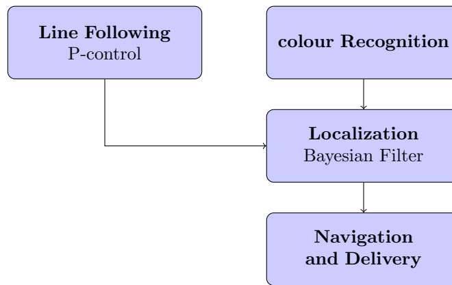
Figure 2: Hierarchy of Sub-tasks
